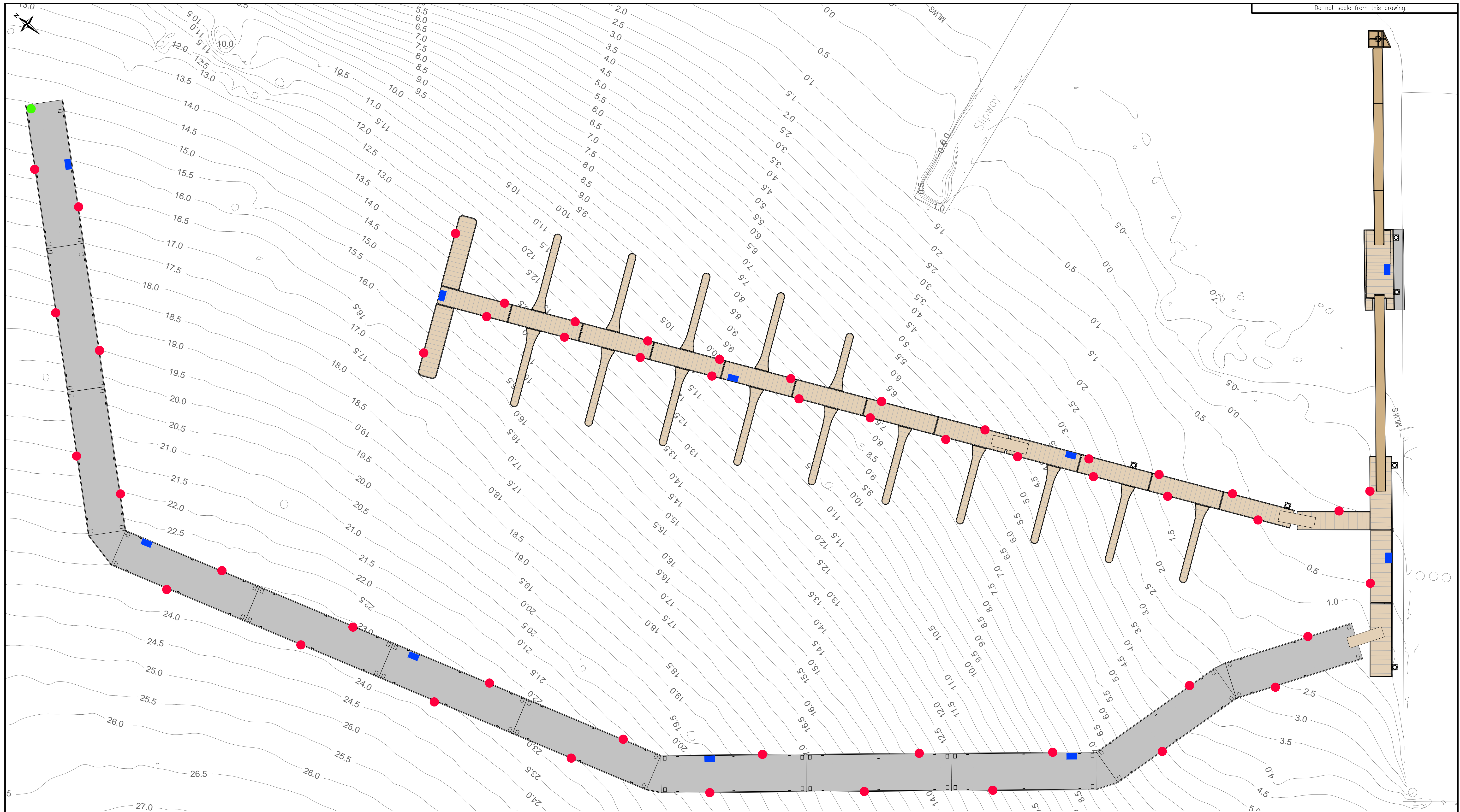
PROPOSED SERVICES LAYOUT PLAN (SCALE 1:250)
